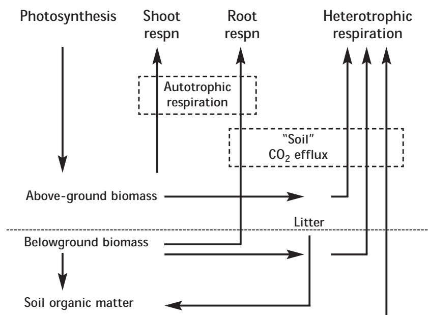
Figure 1: Diagrammatic representation of the main terms describing carbon fluxes in ecosystems.
