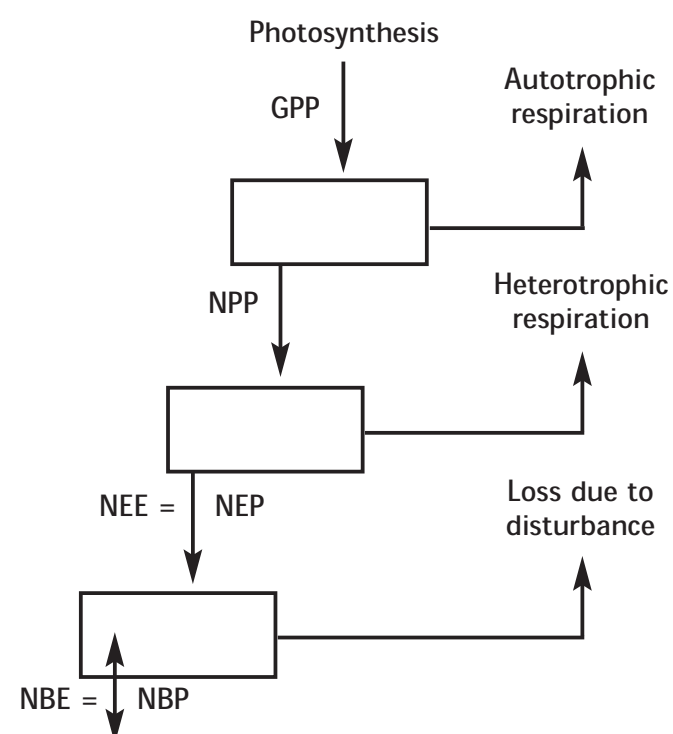
Figure 2: Diagrammatic representation of the main terms describing system carbon balances. Arrows indicate that GPP and NPP are always positive (carbon gains by the system), NEE is usually, but not always, positive, and NBE can be positive or negative.
